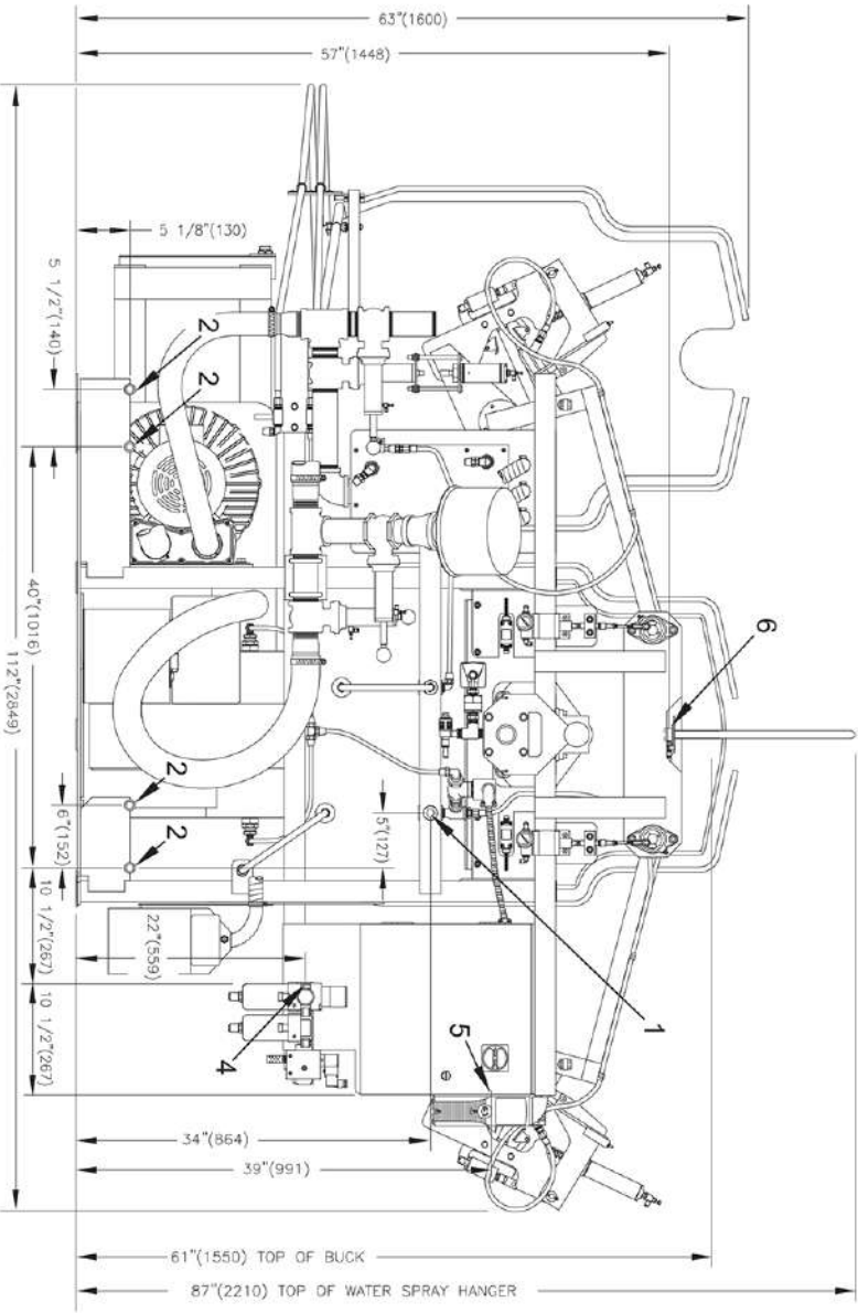
REAR VIEW
