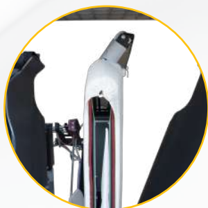
Nuovi piani sagomati teflonati New contoured Teflon-coated bucks
